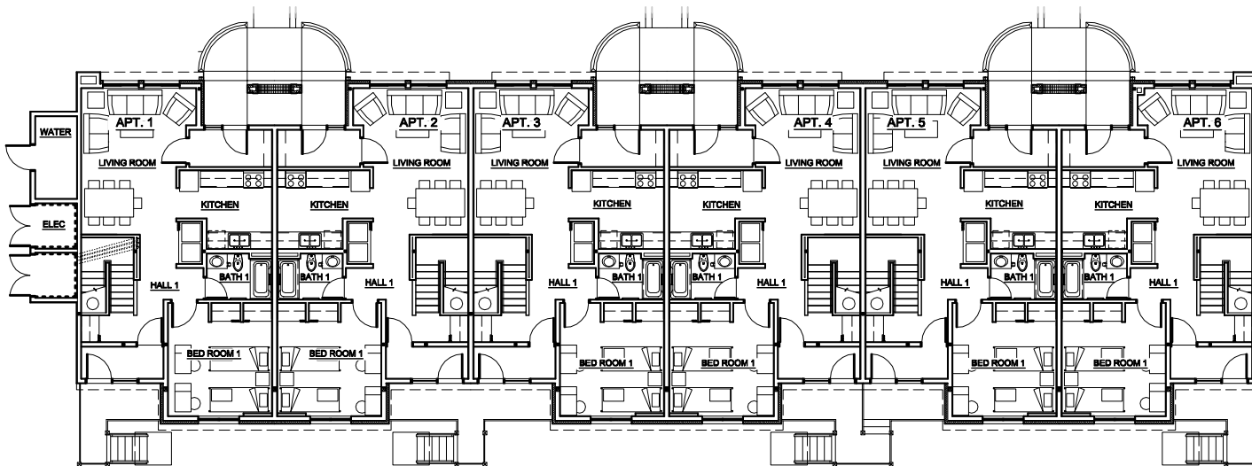
BUILDING "O" FIRST FLOOR PLAN
