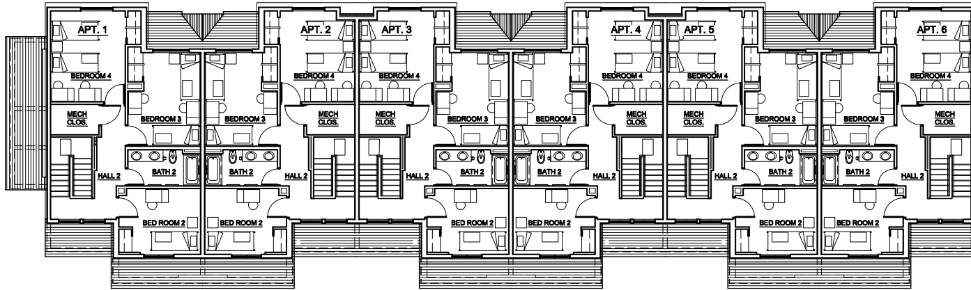
BUILDING "O" SECOND FLOOR PLAN
