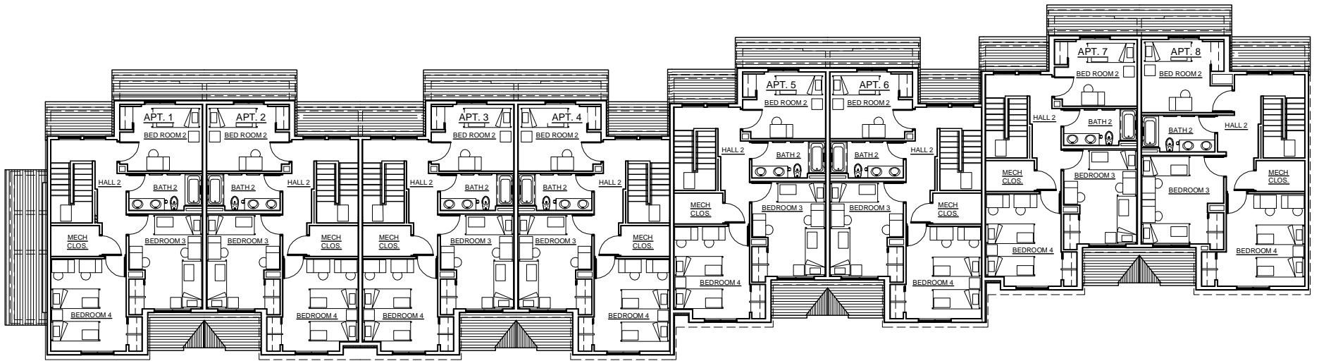
BUILDING "P" SECOND FLOOR PLAN
